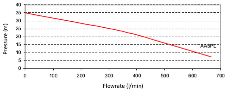
Flow curve for AA5 PL pump
